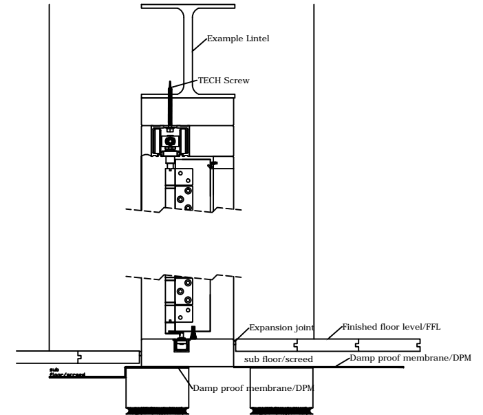
Valdi Ltd - Top Hung Folding Sliding Doors - Conservatory sill (without weather stop)- Timber flooring
