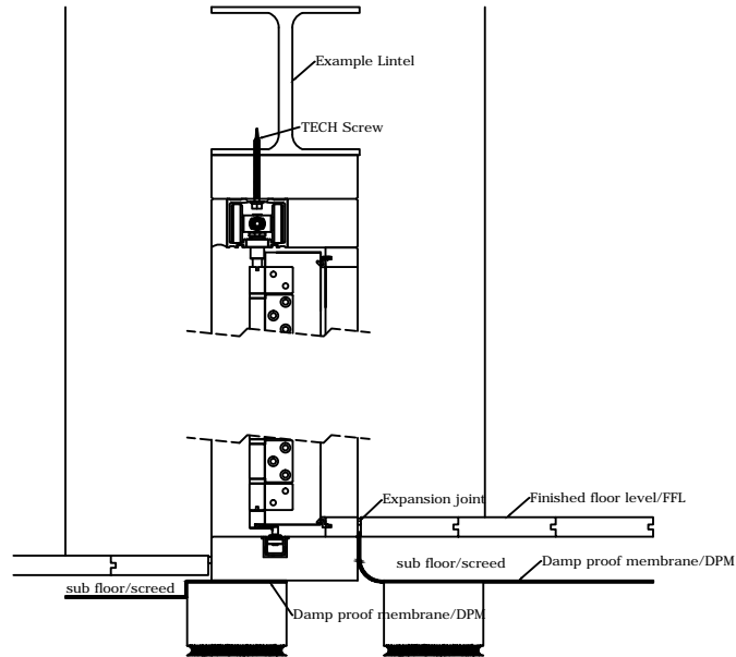
Valdi Ltd - Top Hung Folding Sliding Doors - Conservatory sill (with weather stop)- Timber flooring
