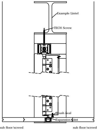
Valdi Ltd - Top Hung Folding Sliding Doors - Room divider sill - Timber flooring
